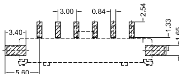
Recommended P.C.B Layout General Tolerance±0.05
