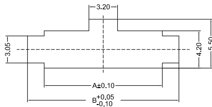
SINGLE ROW RECOMMENDED PANEL CUT-OUT (DESIGNED FOR 1.57mm TO 2.30mm THICK STAMPED PANEL OR PRINTED CIRCUIT BOARD)
