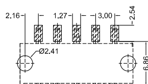
Recommended P.C.B Layout General Tolerance±0.05
