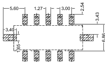
Recommended P.C.B Layout General Tolerance±0.05
