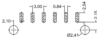
Recommended P.C.B Layout General Tolerance±0.05
