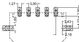
Recommended P.C.B Layout General Tolerance±0.05
