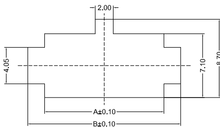
DUAL ROW RECOMMENDED PANEL CUT-OUT (DESIGNED FOR 1.40mm TO 2.54mm THICK STAMPED PANEL OR PRINTED CIRCUIT BOARD)
